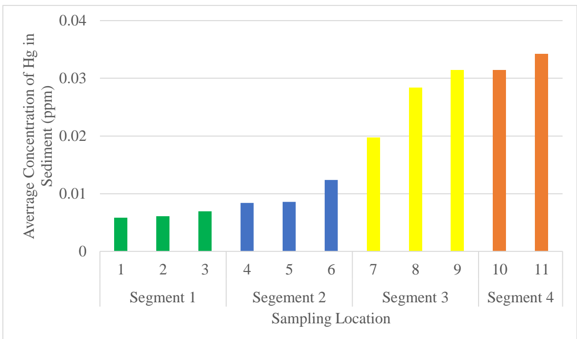
Figure 6. The concentration of Hg in Ciliwung River sediments according to sampling locations
